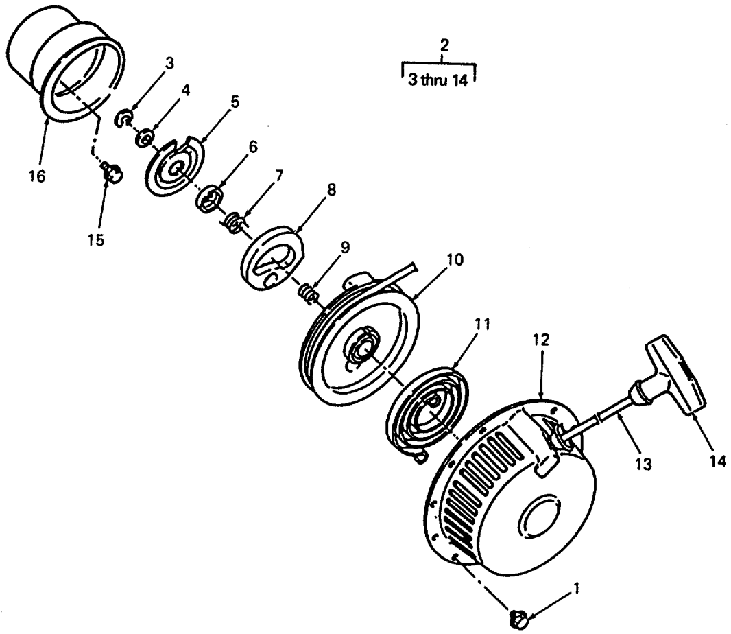
Figure 12. Recoil Starter Assembly
