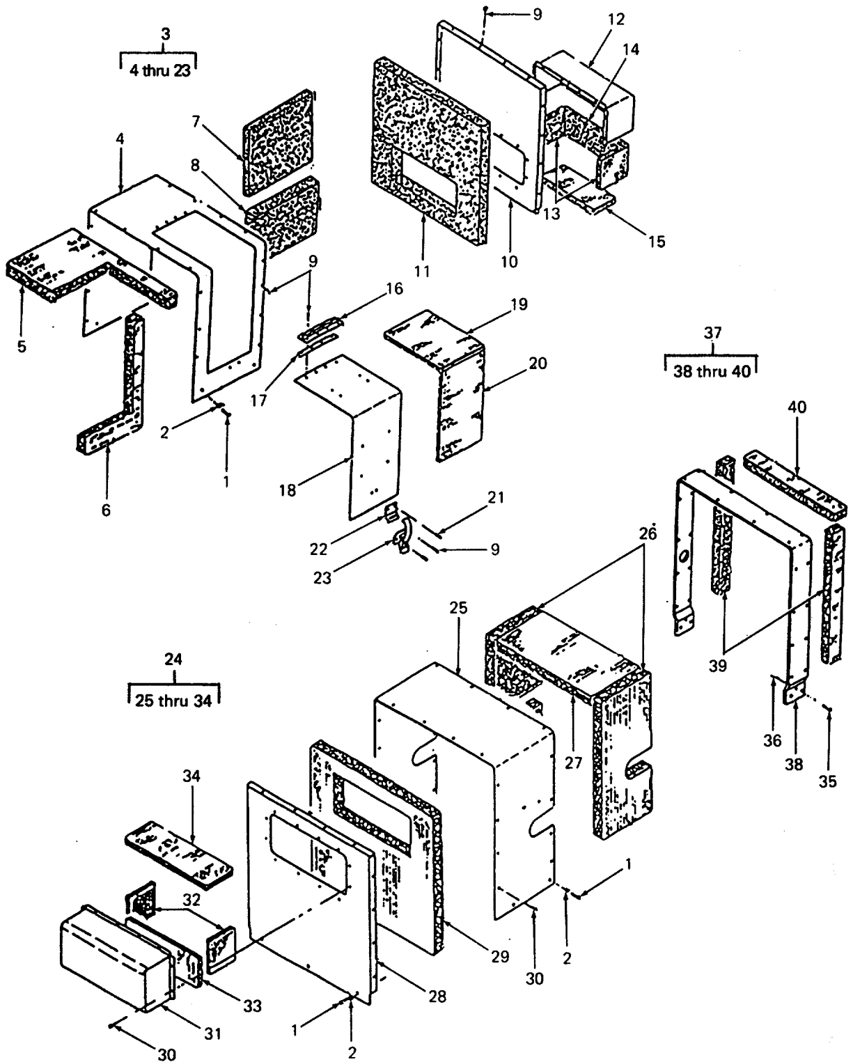
Figure 2. Inlet/Outlet Air Sound Enclosure Assembly
